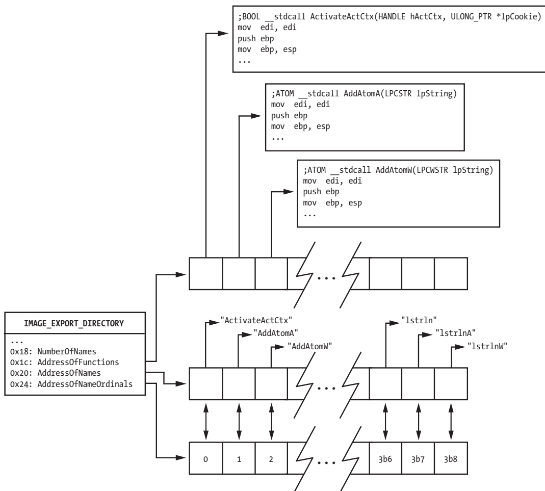
Figure 19-2: kernel32.dll IMAGE_EXPORT_DIRECTORY
