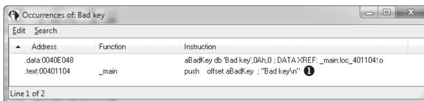
Figure 5-5: Searching example
